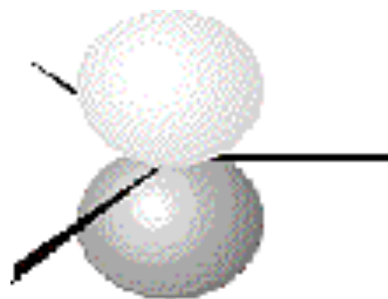
21 AlX_3 and BX_3
