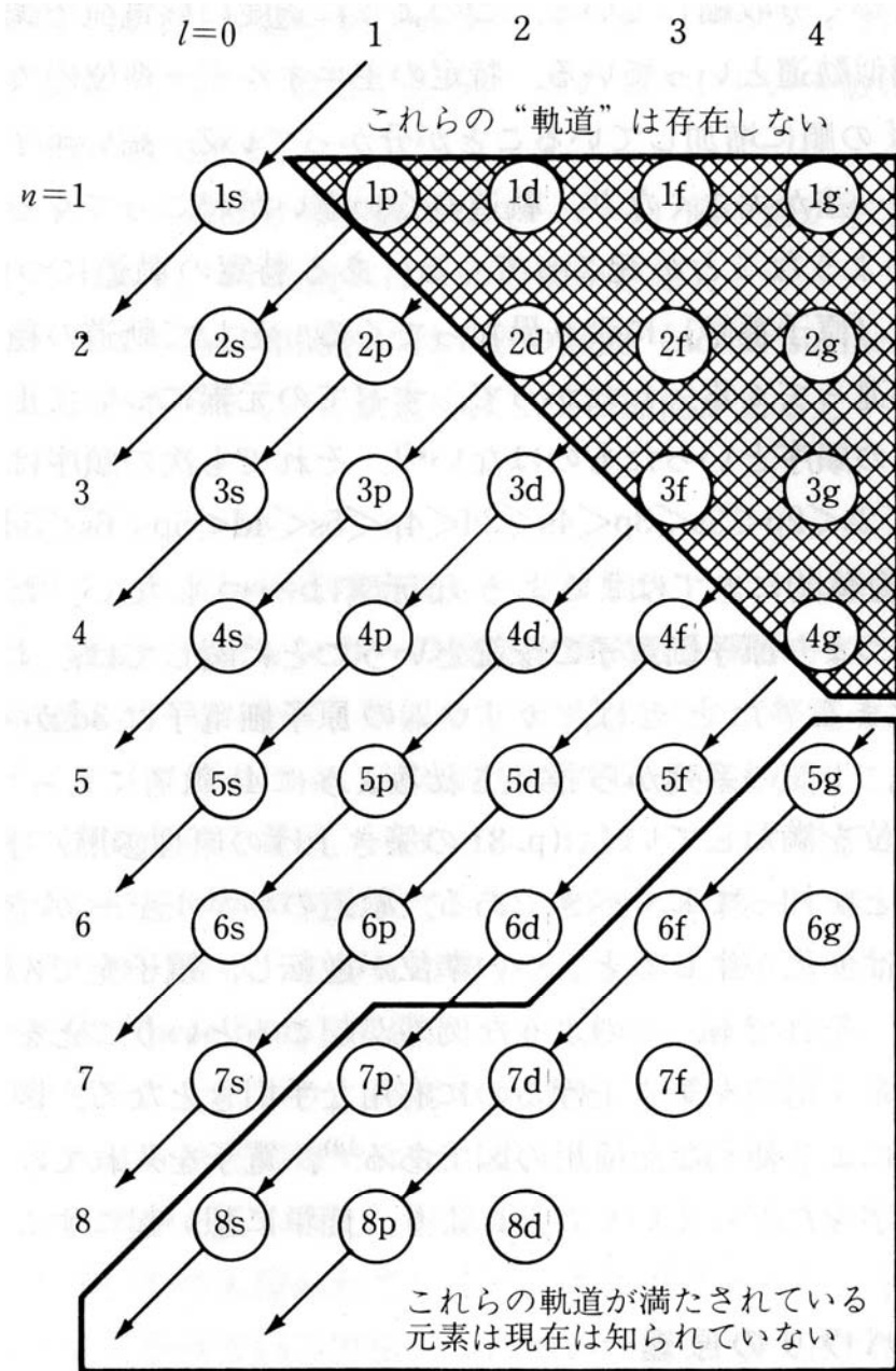
記憶用軌道順序図 (近似的) [T. Moeller, "Inorganic Chemistry," Wiley, New York (1952). 許可を得て転載]
