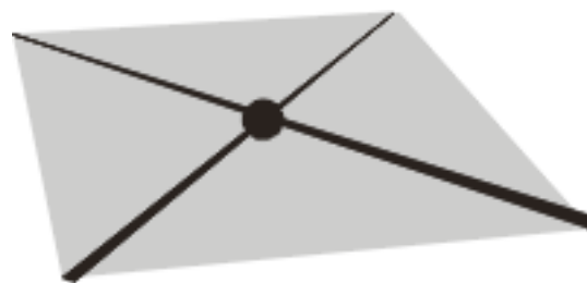
6 Square-planar complex, D_{4h}
