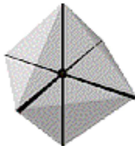
10 Octahedral complex, O_c
